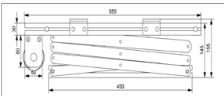
CLOSED LIFT: SIDE VIEW
